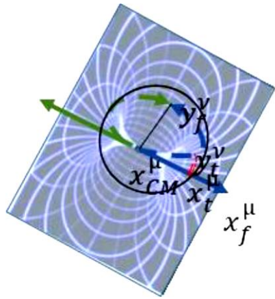
Figure 4: The contribution of \mathcal{PI}_{B_{active}(for: x_{CM(t)}^\mu, t)}(\mathcal{S}, \psi)|_{part(t) \in \mathcal{D}(M)} includes integration over 2\pi . The bundles of fold are sets of tori. Here, we assume: \mathcal{D}(M) = [x_{CM(t)}^\mu, x_t^\mu(part_1)] \cup [x_{CM(t)}^\mu, x_t^\mu(part_2)] .
