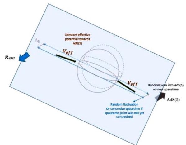
Figure 15: Fluctuations of the position of the entangled particles, result into the attractive effective potential to point towards the tangent dual \text{AdS}(5) space and produce a (constant) force to grow spacetime and hence accelerate expansion. Fluctuations within spacetime only introduce torsion, or fluctuations in spacetime, or concretize not yet existing spacetime as constant rate processes (lattice points never occupied vs. in the first case where new lattice points are created in an accelerated way). The figure illustrates symbolically the 4-D spacetime.
