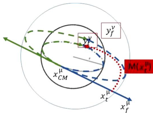
Figure 3: The contribution of \mathcal{PI}_{\mathcal{B}_{active}(\text{for: } x_{CM}^\mu, t)}(S, \psi)|_{(\text{part}(t) \in \mathcal{D}(M))} includes integration over r . Here, we assume:
